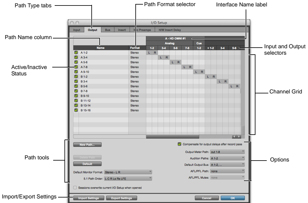
I/O Setup on an HDX system with HD OMNI and HD I/O
