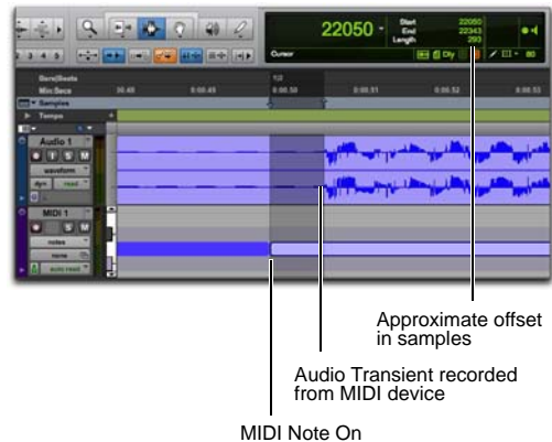
Measuring MIDI latency
